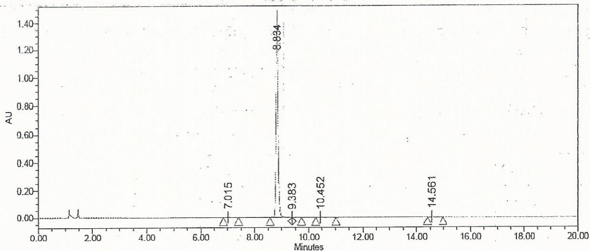
Auto-Scaled Chromatogram
